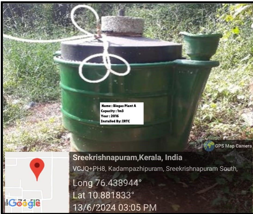
Biogas Plant
